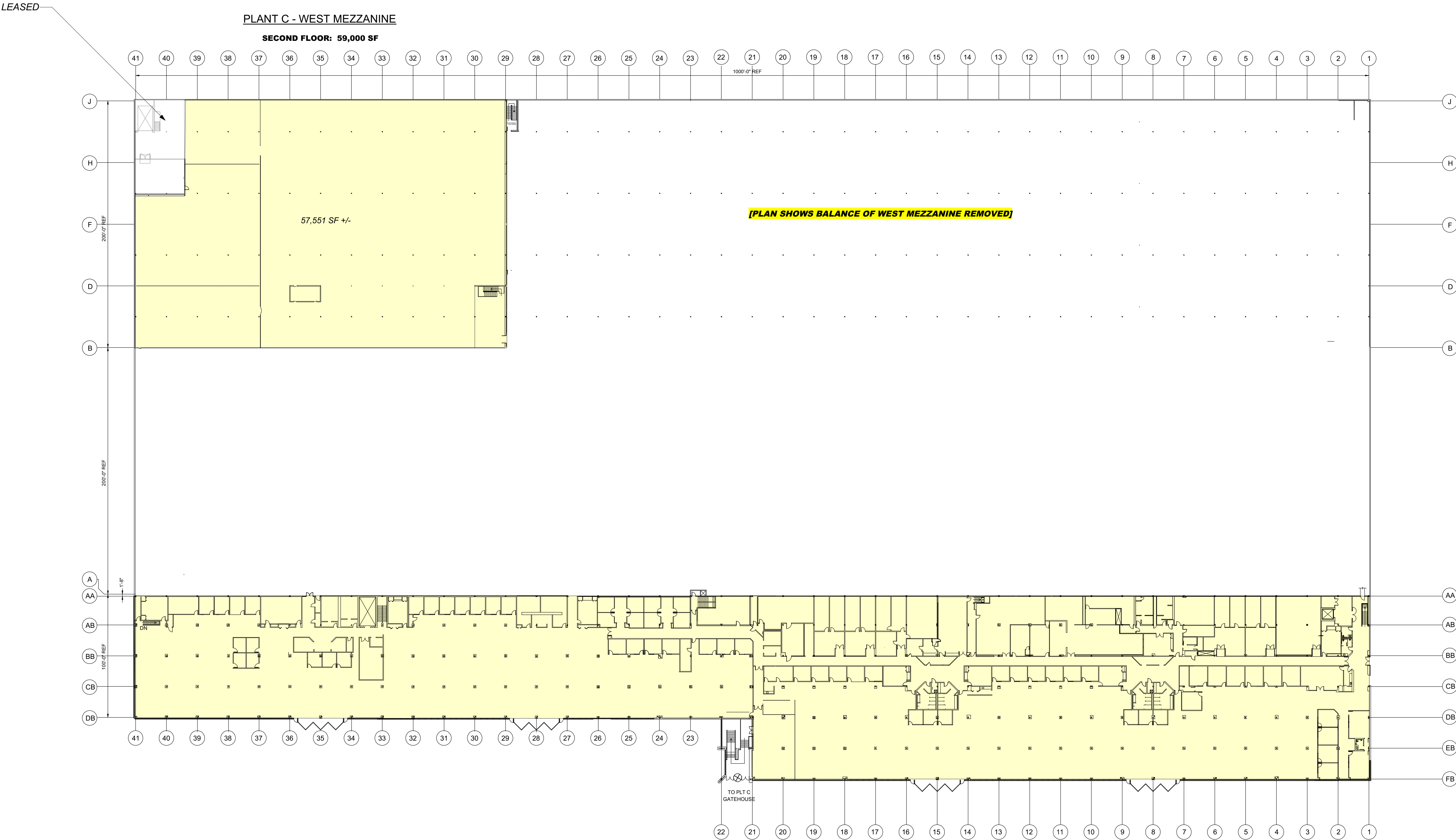
PLANT C - EAST SECOND FLOOR: OFFICE - LAB - TECH 124,000 sf +/-
